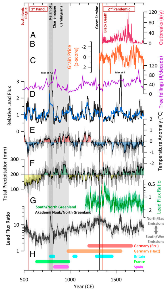
Fig. 4. Arctic lead pollution compared with indicators of plague, economic conditions, and climate from 500 to 1800 CE: (A) number of plague outbreaks per year (29), (B) average European grain prices (11), (C) tree fellingings per decade from historical construction timbers (12), (D) relative lead pollution flux in NG (blue) and AN (black) calculated by subtracting a 600-y spline fit from the log-transformed deposition records, (E and F) reconstructed north central European (E) temperature anomaly (41) and (F) precipitation (23), (G) SG/NG and AN/NG lead flux ratios, and (H) approximate location and periods of known medieval and Early Modern mining activity.
