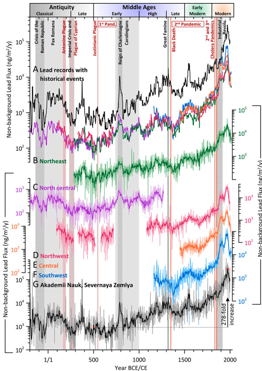
Fig. 1. Annual lead pollution deposition during the past 2,200 y documented in an array of ice cores spanning nearly half the Arctic, including 12 ice cores from Greenland and 1 from Severnaya Zemlya in the Russian Arctic ( SI Appendix, Fig. S1 ). (A) Median filtered (11-y) AN record from Severnaya Zemlya and Greenland regional composite records (records and colors same as in B–G) on the same logarithmic scale. (B–F) Individual Greenland regional composites (annual and 11-y median filtered values shown with thin and thick lines, respectively). (G) AN record from Severnaya Zemlya. The individual Greenland ice core records ( SI Appendix, Fig. S1 and Table S1 ) were grouped by location and regional records of annual concentration ( SI Appendix, Fig. S2 ), flux, and enrichment ( SI Appendix, Fig. S3 ) were computed as the geometric mean of the individual ice core records. The ACT2 (4) and the 200 BCE to 800 CE part of the NGRIP2 (2) record have been published previously ( SI Appendix, Table S1 ). Measurements in the few previously reported Arctic lead measurements (3–5), all confined to the central region of the Greenland ice sheet, are consistent with the records presented here ( SI Appendix, Fig. S2 ). Because accurate dating of ice core records is critical for meaningful historical interpretation, all cores were volcanically synchronized to an accurately dated Arctic reference record ( Materials and Methods ). Uncertainties in the individual core chronologies were estimated to be <2 y (2) for the Greenland records and <5 y for the AN core ( Materials and Methods ). Widespread pollution increased more than 250-fold from the Early Middle Ages to 1970s, with sharp, often sustained increases coincident with periods of political stability (e.g., early Carolingian Empire) and exploitation of new mining regions, and decreases coincident with plagues (e.g., Black Death, second plague pandemic from 1348 to ~1700 CE; second cholera pandemic from 1829 to 1837 CE; third cholera pandemic from 1846 to 1860 CE), climate (e.g., Little Ice Age), major wars, and other externalities. Similar variability throughout the Arctic array indicates large-scale, common changes in lead emissions.
