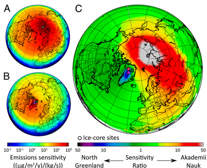
Fig. 3. FLEXPART (18, 19) simulation-based sensitivity of the (A) AN and (B) NG ice core records to lead emissions and (C) their ratio. The ~8-fold higher lead deposition observed in the AN record compared with the NG composite (Fig. 1) is consistent with the 2- to 12-times higher sensitivity to European emissions in the AN/NG ratio, indicating that lead pollution in the Arctic array was dominated by European emissions before the Industrial Revolution.
