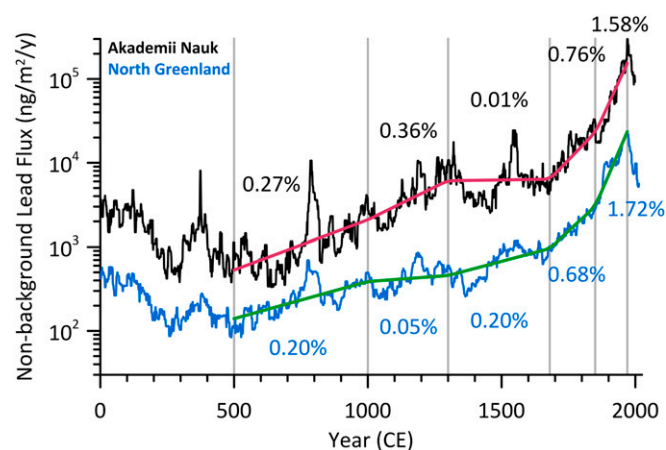
Fig. 2. Arctic lead pollution (11-y median filter) with fitted average growth rates ( Materials and Methods ) during specific historical periods in the NG (green) and AN (red) records ( SI Appendix, Table S2 ).
